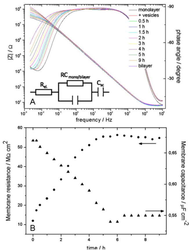
FIG. 7. (Color online) Vesicle fusion monitored by EIS on a DPhyTL-based tBLM. (a) The spectra in the Bode plot show an increase in resistance after vesicle addition. (b) The fitted resistance and capacitance values are depicted as a function of time. An increase in resistance and a capacitance drop can be seen.
